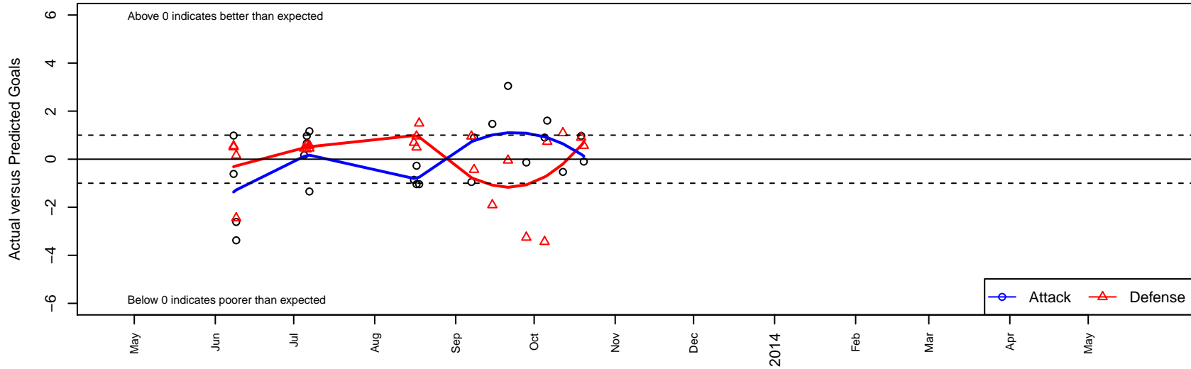
Basin Utd Fusion–Gold G00 Dots are actual minus expected GF (blue circles) and GA (red triangles). Blue line is smoothed change in attack strength. Red is smoothed change in defense strength.
